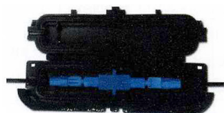
B1-DMINA02 (Splicing 1 fibers) Outdoor wall mounted, Can load SC fast connector or mechanical splicer (160x48.2x16mm)
