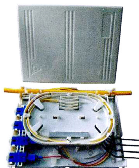
B1-BC04C (Splicing 8 Fiber) Indoor wall mounted, cable entry without cutting, Can load PLC 1:4 splitter & 4 pcs mechanical splicers (130x180x30.4mm)
