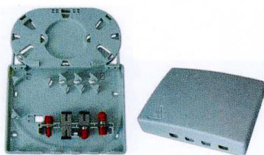
B1-BC04 (Splicing 4 fibers) Indoor wall mounted (150x110x34mm)
