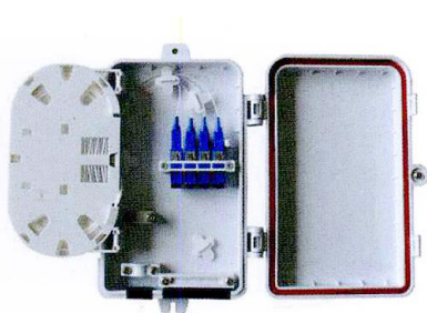
B1-BC04A (Splicing 8 Fiber) Outdoor wall mounted, Pole mounted optical, Can load PLC 1:4 splitter (141.6x211.6x39.8mm)
