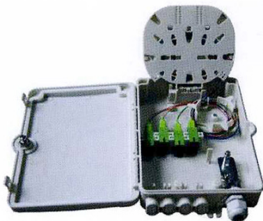
B1-BP08 (Splicing 8 Fiber) Outdoor Wall mounted & Poles mounted, Can load PLC 1:4, 1:8 splitter (171.4x234.5x47.4mm)
