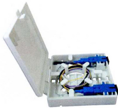
B1-G009A (Splicing 2 Fiber) with hinged cover
