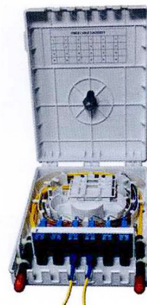
B1-BR24 (Splicing 24 Fiber) Indoor wall mounted, cable entry without cutting, two modules: the one is for max. 24 fiber splicing, the other is for 1 PLC-1:16 splitter & 8 fiber splicing (193x246.5x53.2mm)
