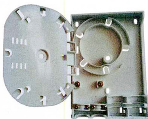
B1-BC04E (Splicing 4 Fibers) Indoor wall mounted, cable entry without cutting (90x124x22mm)
