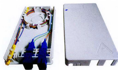
B1-BC04D (Splicing 8 Fiber) Indoor wall mounted, cable entry without cutting, Can load PLC 1:4 splitter (90x165.73x24.1mm)
